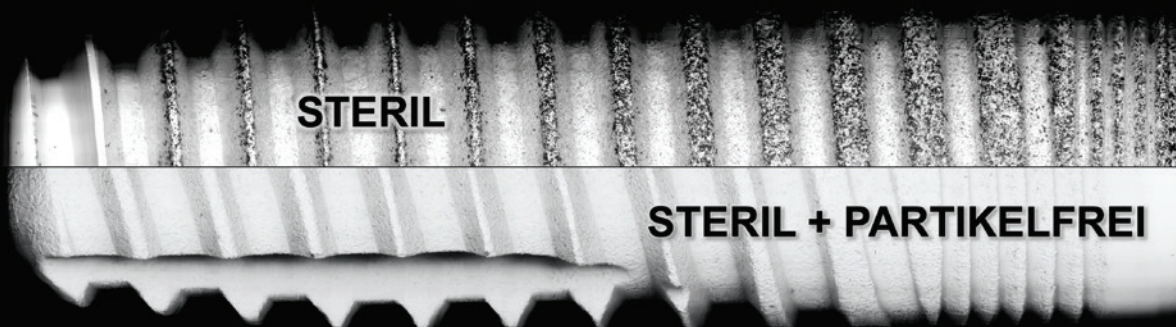
Full-size high-resolution SEM image mapping Backscattered electron imaging 500x
