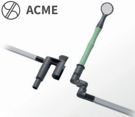
Functional UHD Dental Mirror combined with LED, Endo-Gauge, AirClean, Photography and Suction.
