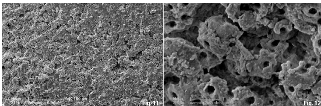
Figs. 11 & 12_ SEM images of radiated dentine with diode 810 nm laser (dry, 1.5 W, 15 Hz) with 50% ton-toff and 200 µm fibre, showing evidence of thermal effects, with detachment and smear layer.
