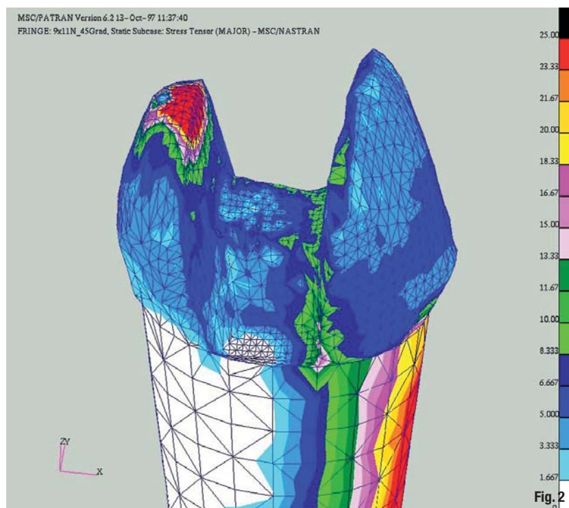
Fig. 2 Finite element measurement with the exertion of chewing forces: the ceramic inlay bears the chewing load; the tooth substance remains stress free (inlay is hidden). (Illustration: Prof Albert Mehl)
