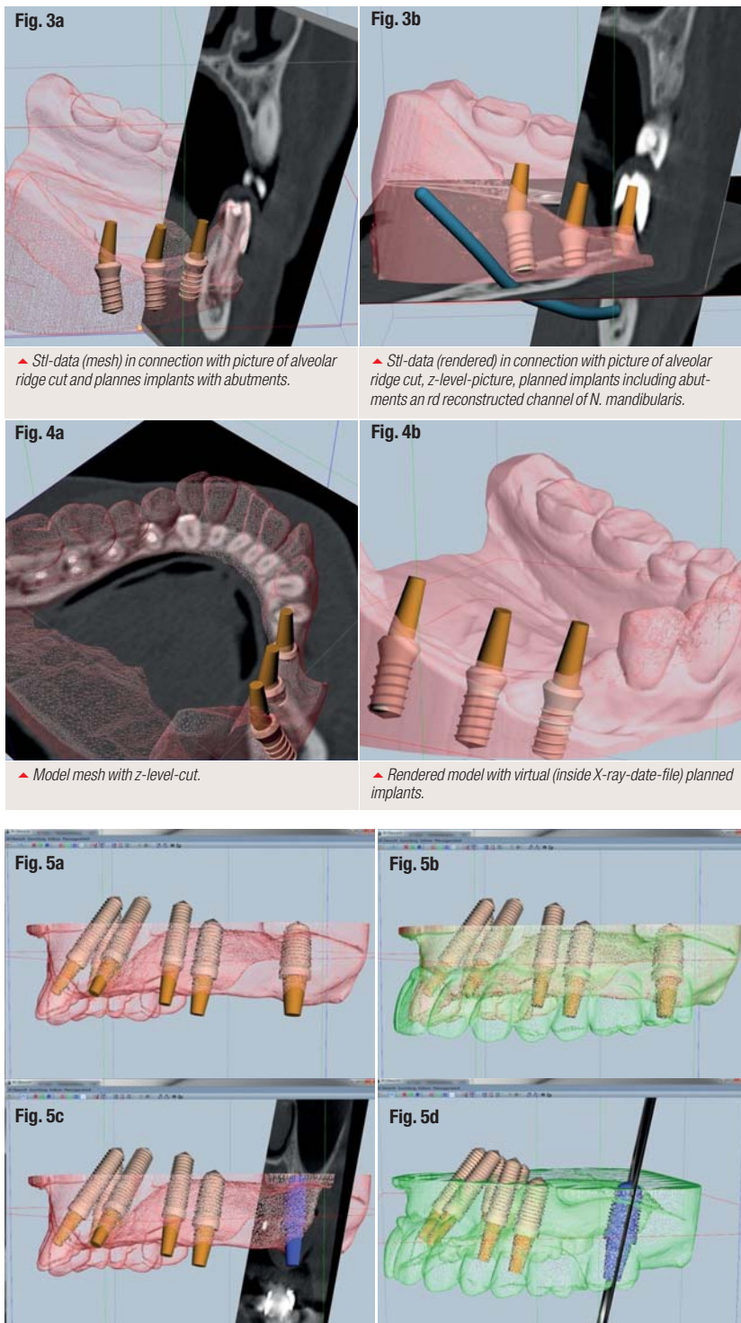
Figs. 3a–b & 4a–b A selection of the options for merging the optical scan of the model with 3-D radiological planning data. Figs. 5a–d Merging the optical scan of the model (red) with an aesthetic set-up (green) using 3-D radiological planning data.
