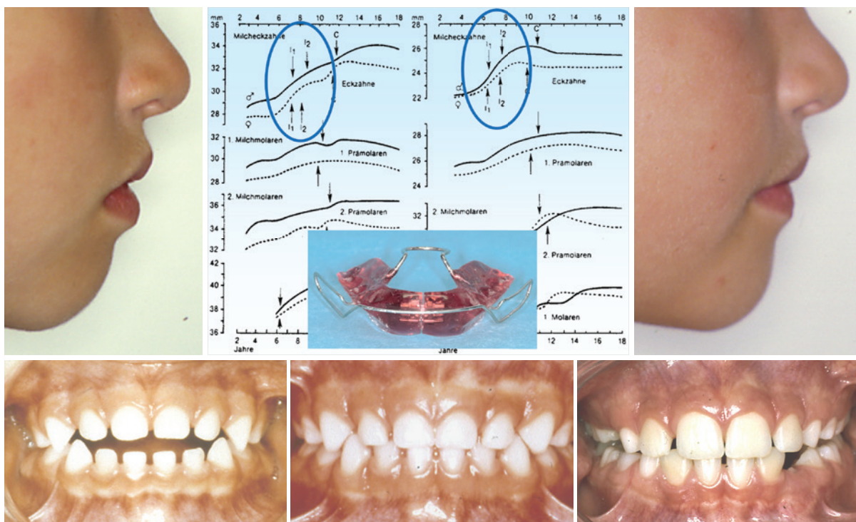
Moorrees-Kurven
