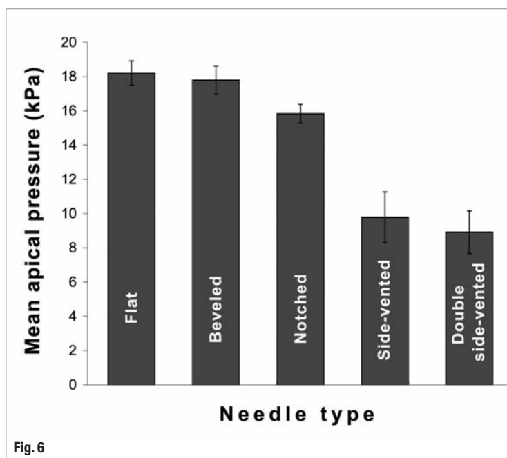
Fig. 6 Time-averaged irrigant pressure at the apical foramen for various needle types: open-ended (A–C), closed-ended (D & E). Data shown as mean \pm standard deviation. (Reprinted with permission from Boutsioukis et al. 2010b.)
