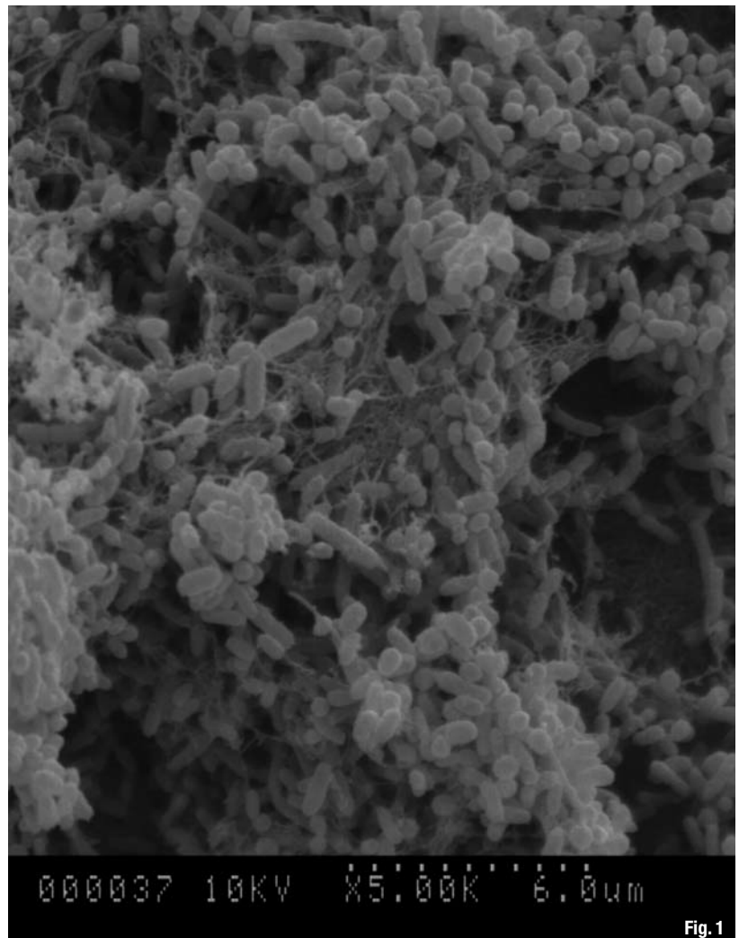
Fig. 1 Multispecies bacterial biofilm grown on root-canal dentine in vitro .
