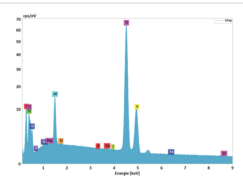
Fig. 1: Integrated spectrum across the entire imaged area. C = carbon; Ti = titanium; N = nitrogen; O = oxygen; F = fluorine; Na = sodium; Mg = magnesium; Al = aluminium; Si = silicone; K = potassium; Ca = calcium; I = iodine; V = vanadium; Fe = iron; Zn = zinc.
